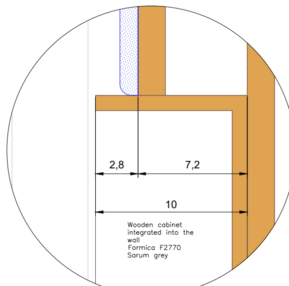
Detail 02 - Cabinet - niche Scale 1:5
